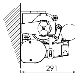
Montaggio a parete Wall installation
