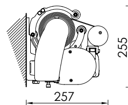
Montaggio a parete Wall installation
