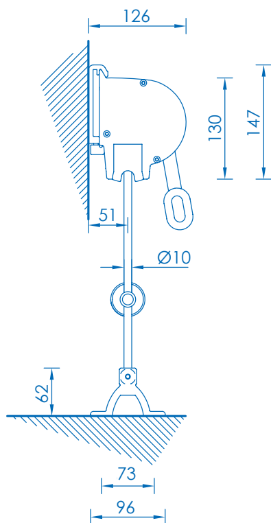
Montaggio a parete Wall installation
